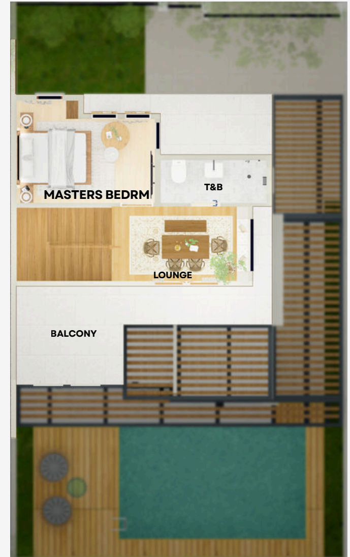
Third Floor Plan - 41.98 sqm Floor Area
